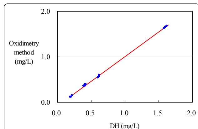
Figure 4 Oxidimetry and electrochemical methods for DO-unregulated hydrogen water. Value obtained by the oxidimetry method = -0.0837 + 1.0829 \times value obtained by the electrochemical method.
